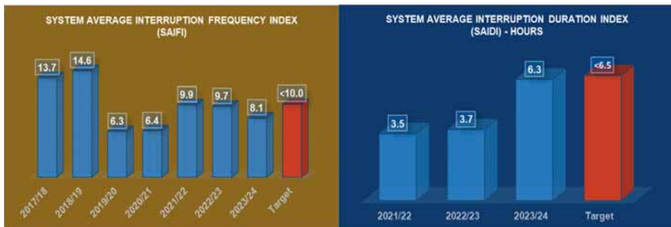
Figure 51: Performance of Electricity Transmission Infrastructure Reliability Indices
