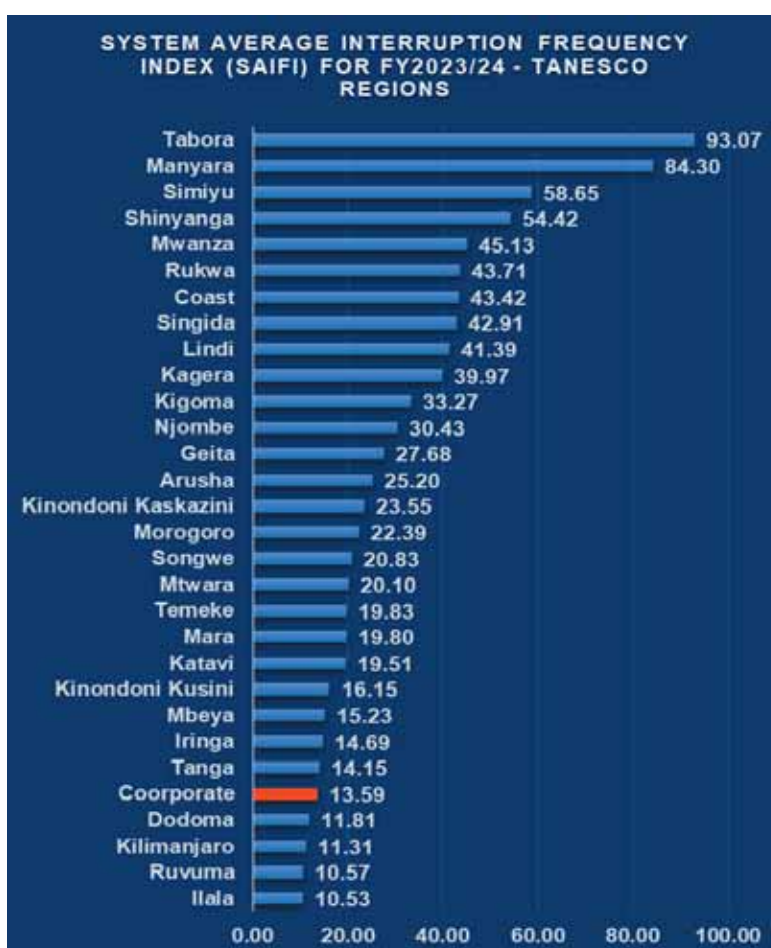
Figure 65: System Average Interruption Frequency Index (SAIFI) in FY 2023/24 – TANESCO Regions
