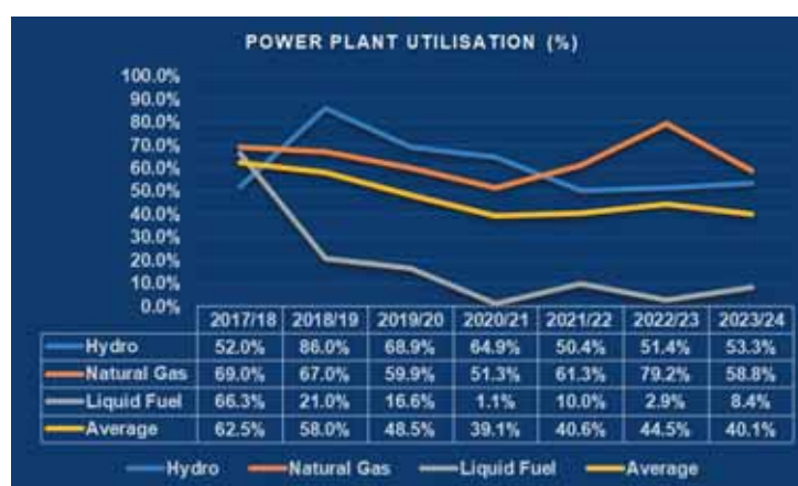
Figure 42: Power Plant Utilization (%)
